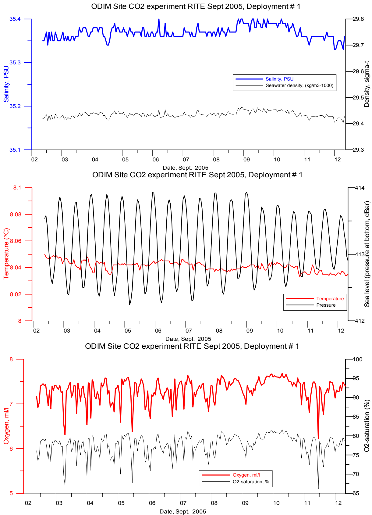
Figure 10. Time series of hydrographic data from 400 m depth at Storffjorden during 02-12 September, 2005.
