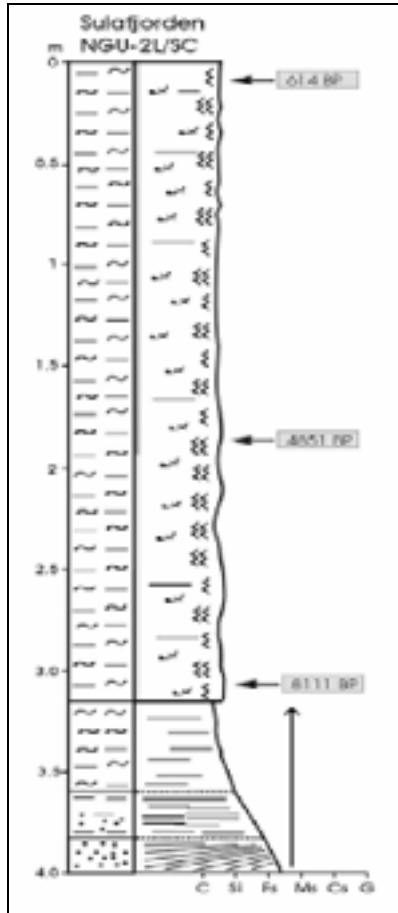
Figure 4. Left: Lithology of a sediment core from Storffjorden (Sulafjorden). Right: Sediment profile from same location. From Bøe et al. 2004.
