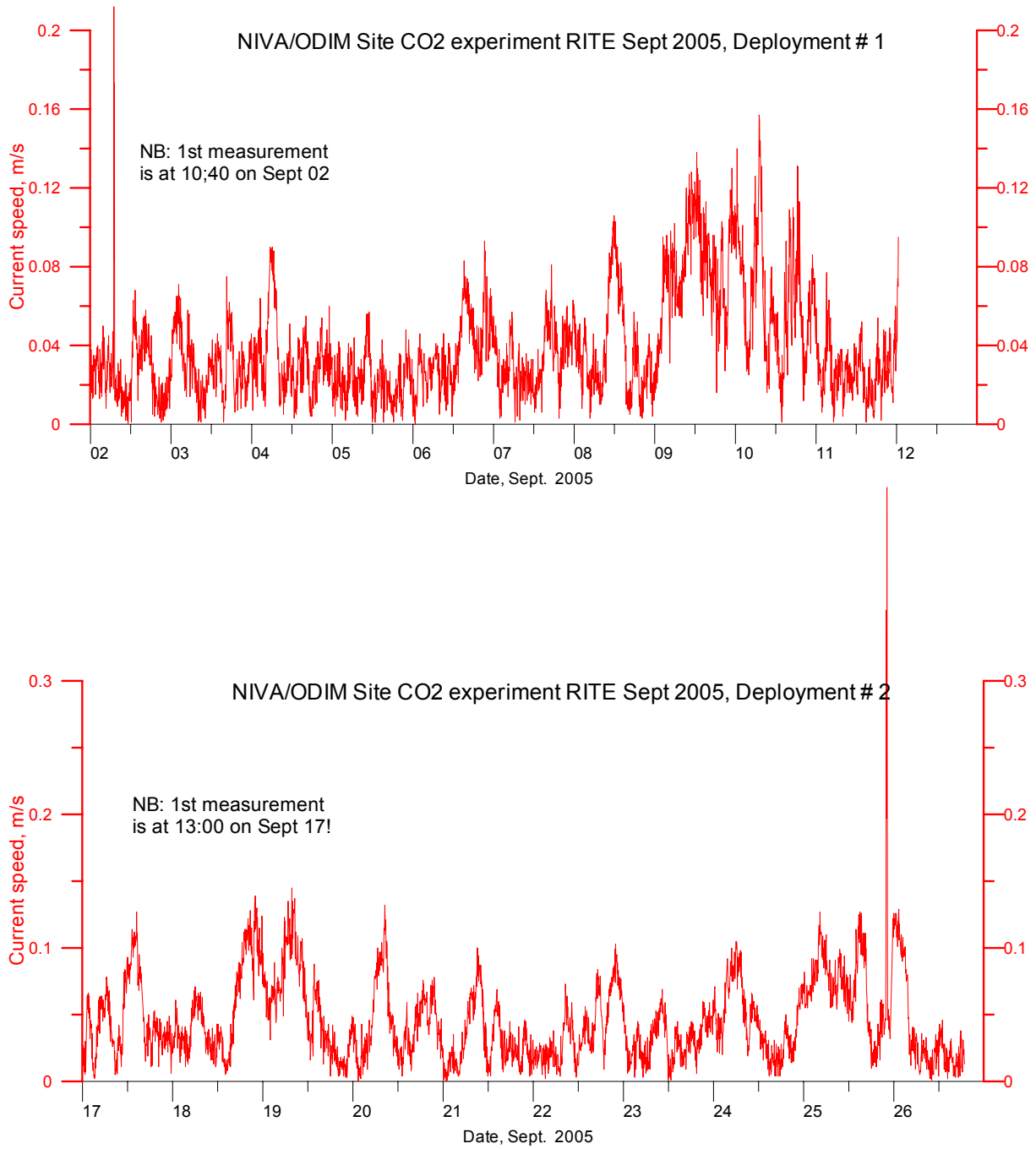
Figure 11. Measured current speed 3 m above the bottom at 400 m depth in Storjorden, 17-27 September 2005.
