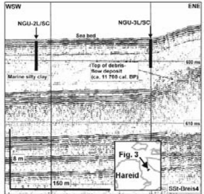
Fig. 3. Seismic profile (Sparker) with core locations, Sulafjorden. A sound velocity of 1600 m/s was used for conversion of milliseconds to meters. Vertical exaggeration ca. \times 10 . See inset map and Fig. 1 for location.
